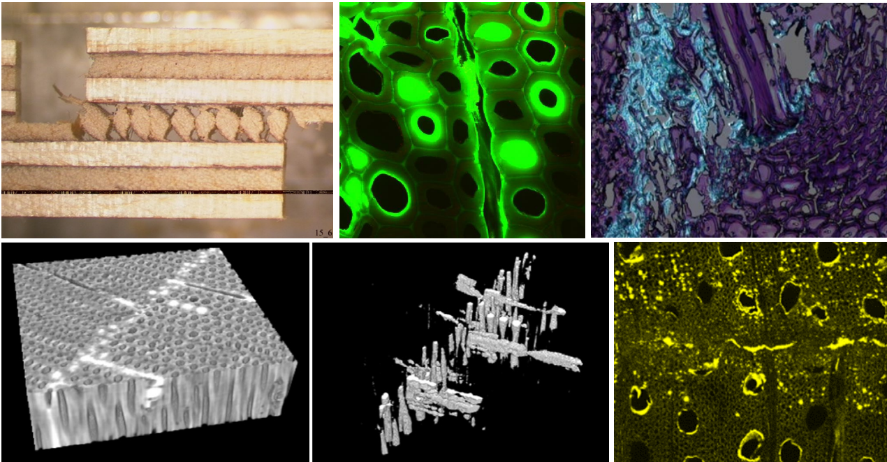
Top: Plywood shear, deep lathe checks pulled open; Green fluorescent PF in veneer; Light blue UF in particleboard. Bottom: X-ray tomographic visualization of adhesive penetration, with and without wood shown; pMDI bondline. Photo credits: Anti Rohumaa, Chris Hunt and Warren Grigsby, Hogger Elfriede, Joseph Jakes, Ning Yan
