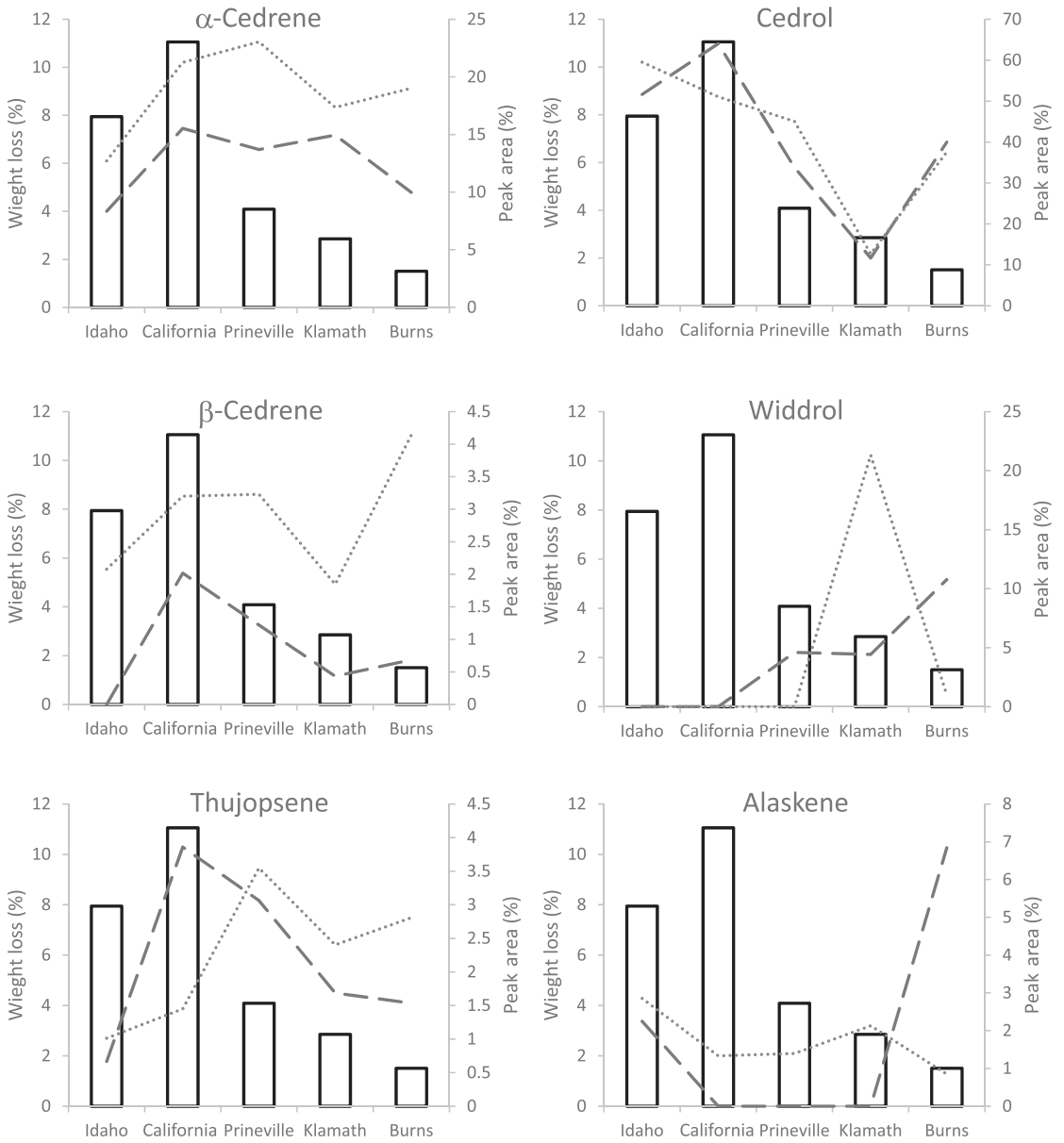
Figure 3. Average extractive contents for hexane (dashed line) and methanol (dotted line) extracts from western juniper heartwood samples from five different geographic sources compared with mass loss caused by exposure to Gloeophyllum trabeum in an American Wood Protection Association soil block test (black hollow bars).
